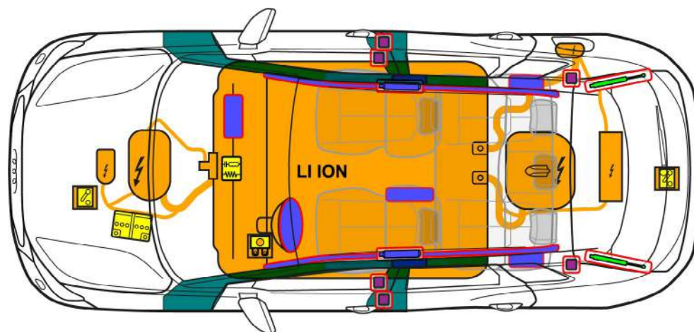
Rescue sheet for the Audi Q4 e-tron
